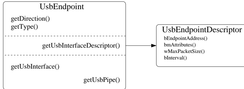
Figure 6: UsbEndpoint
