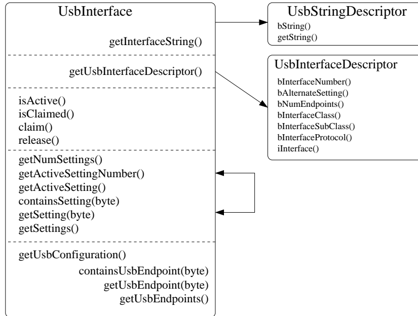
Figure 5: UsbInterface
