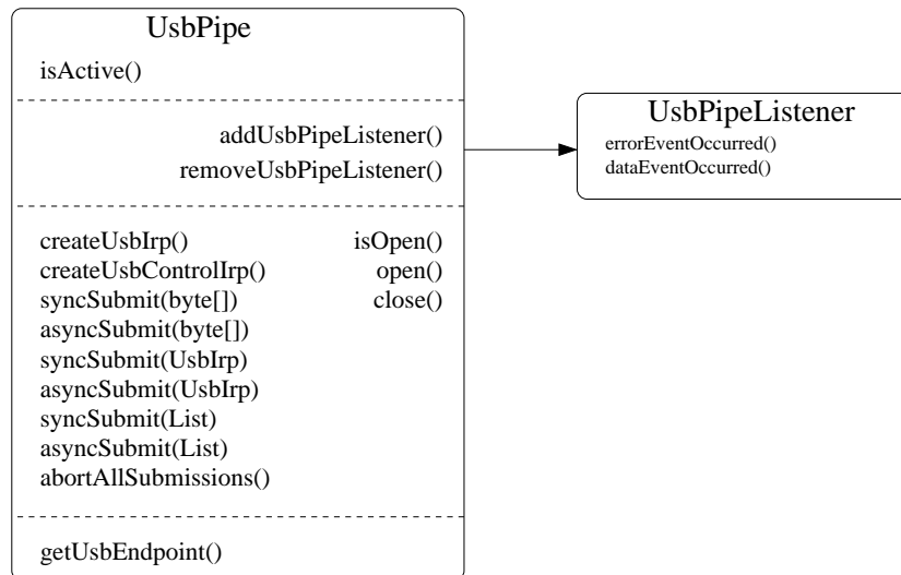
Figure 7: UsbPipe
