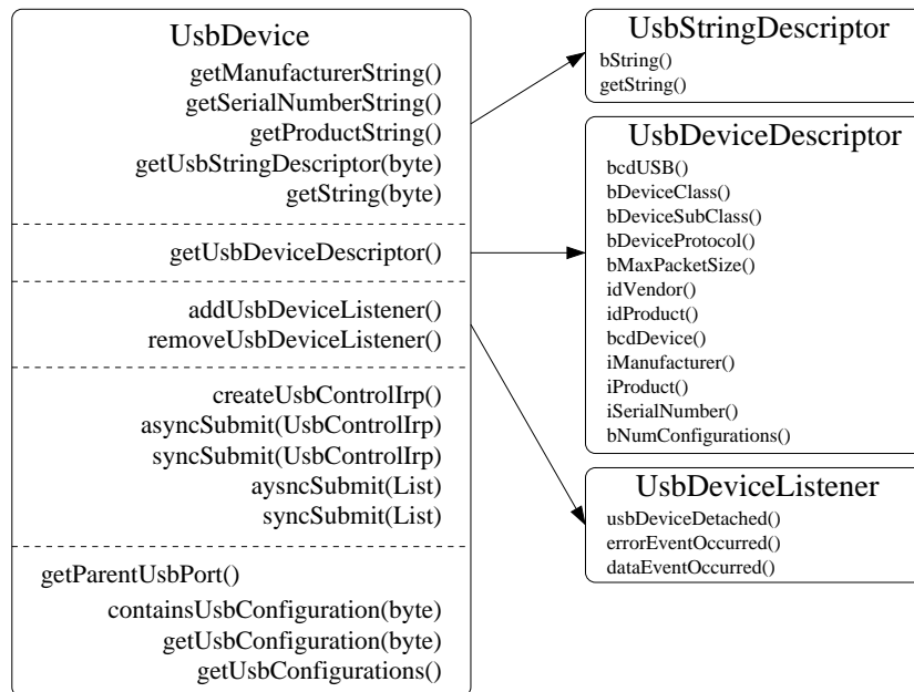
Figure 3: UsbDevice
